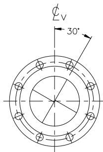
UPSTREAM END VIEW
