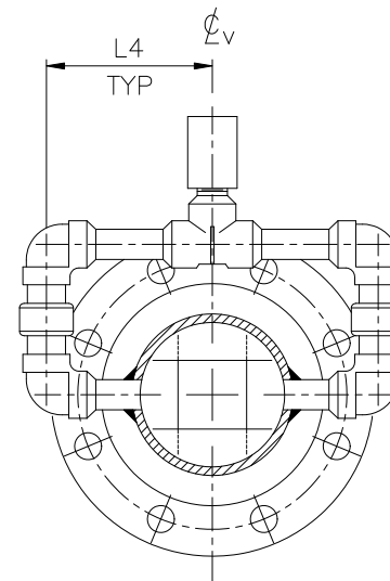
SECTION THRU A
