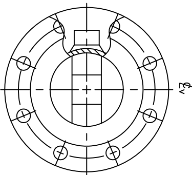
DOWNSTREAM END VIEW
